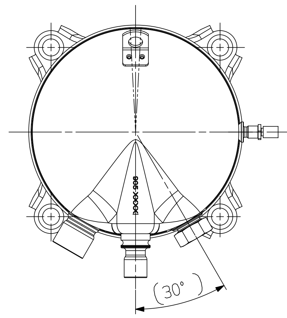
SIGHT GLASS LAYOUT T-BOX REMOVED
